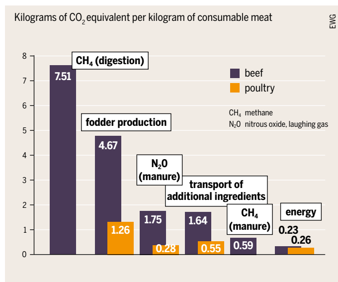
Emissions from meat production in the USA
