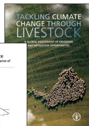
FAO report: Climate change through livestock, 2013
